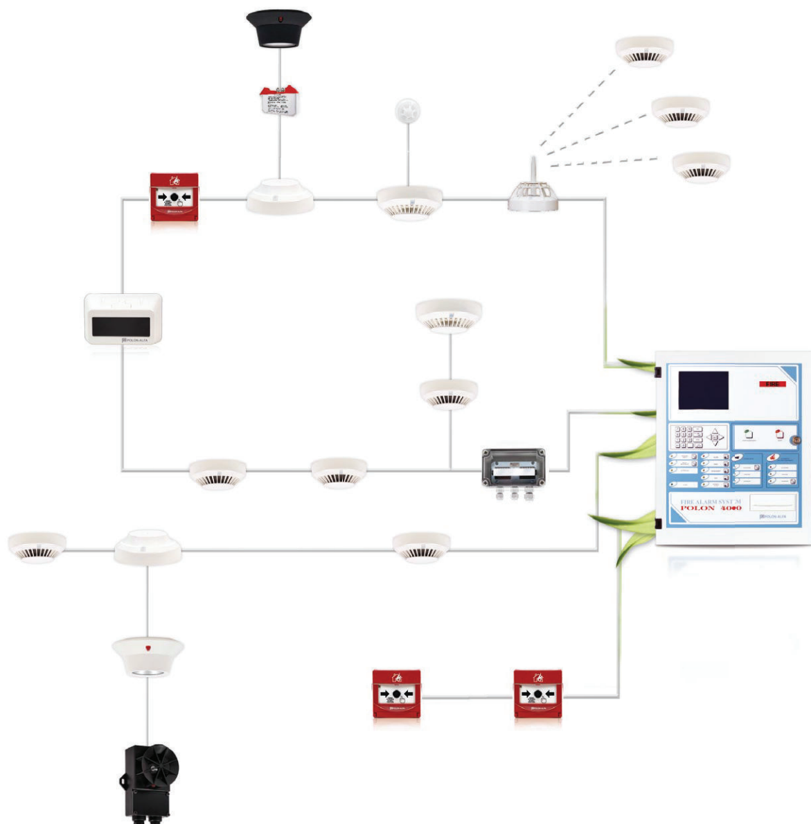
Detector lines of POLON 4200 control panel
