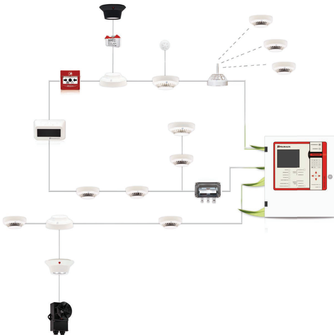
Detector lines of POLON 4100 control panel
